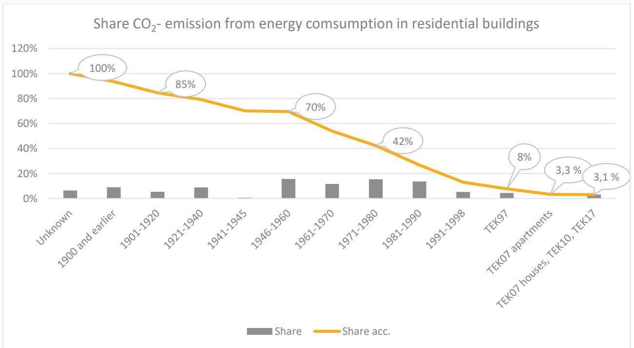
Figure 6 The building stock’s relative share of CO 2 –emissions related to energy demand dependent on building year and code (Statistics Norway and Multiconsult)
