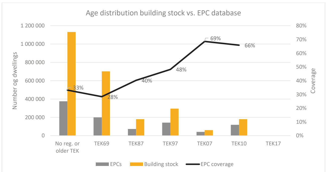
Figure 9 Age distribution in Energy Performance Certificates vs. actual residential building stock and EPC coverage by building year (Source: energimerking.no and Statistics Norway, August 2019)
